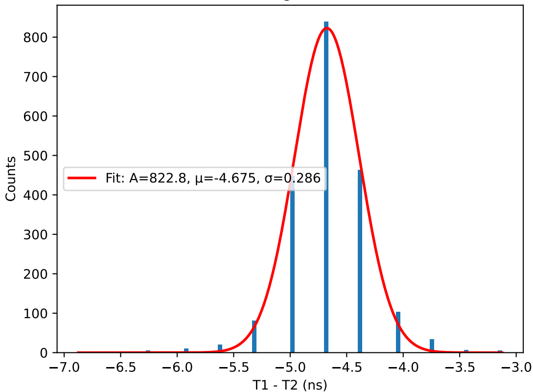
T1 - T2 histogram for 45.0V
