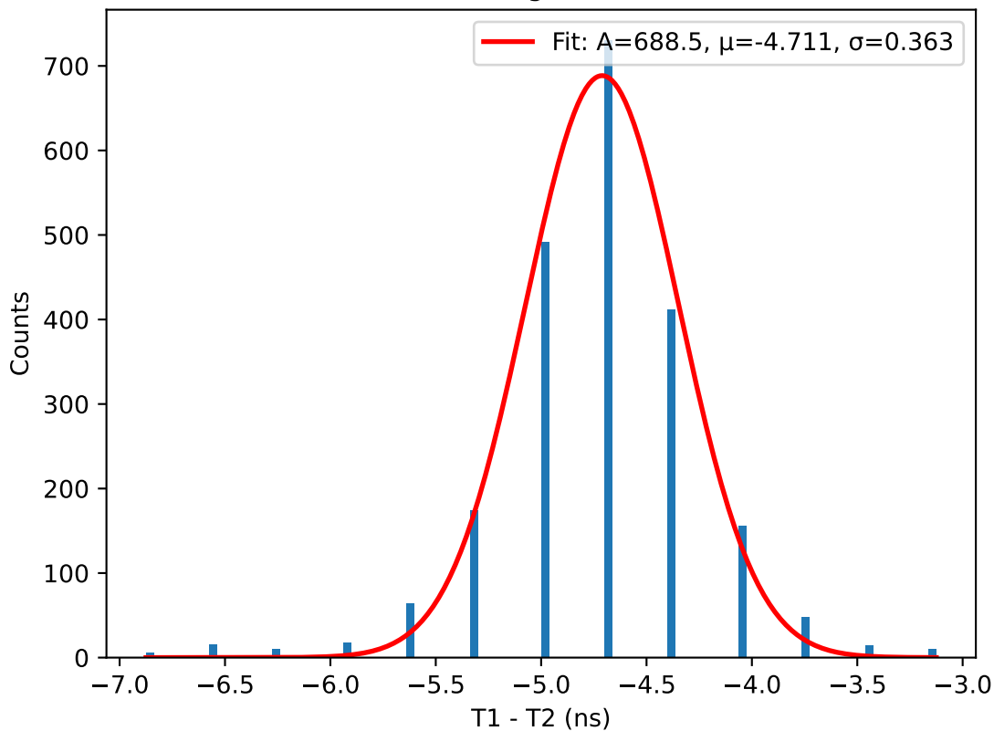
T1 - T2 histogram for 42.0V
