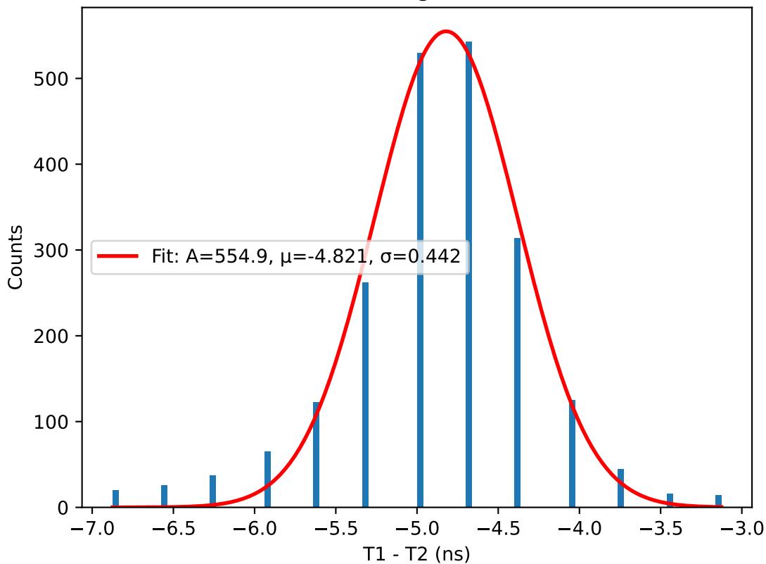
T1 - T2 histogram for 41V
