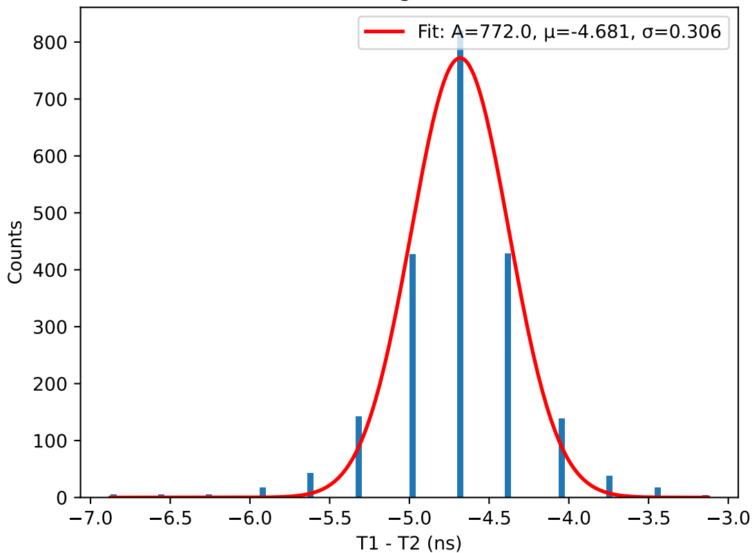
T1 - T2 histogram for 43.0V
