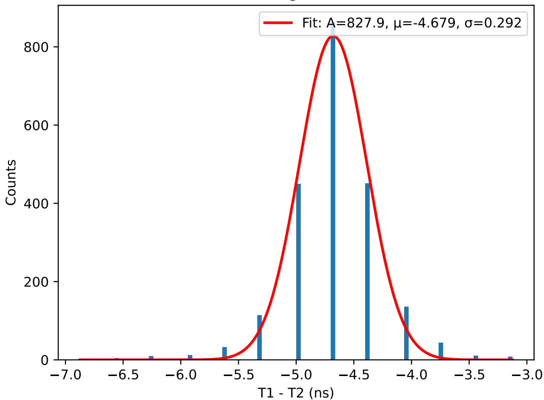
T1 - T2 histogram for 43.5V
