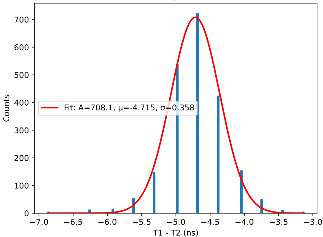
T1 - T2 histogram for 42.5V
