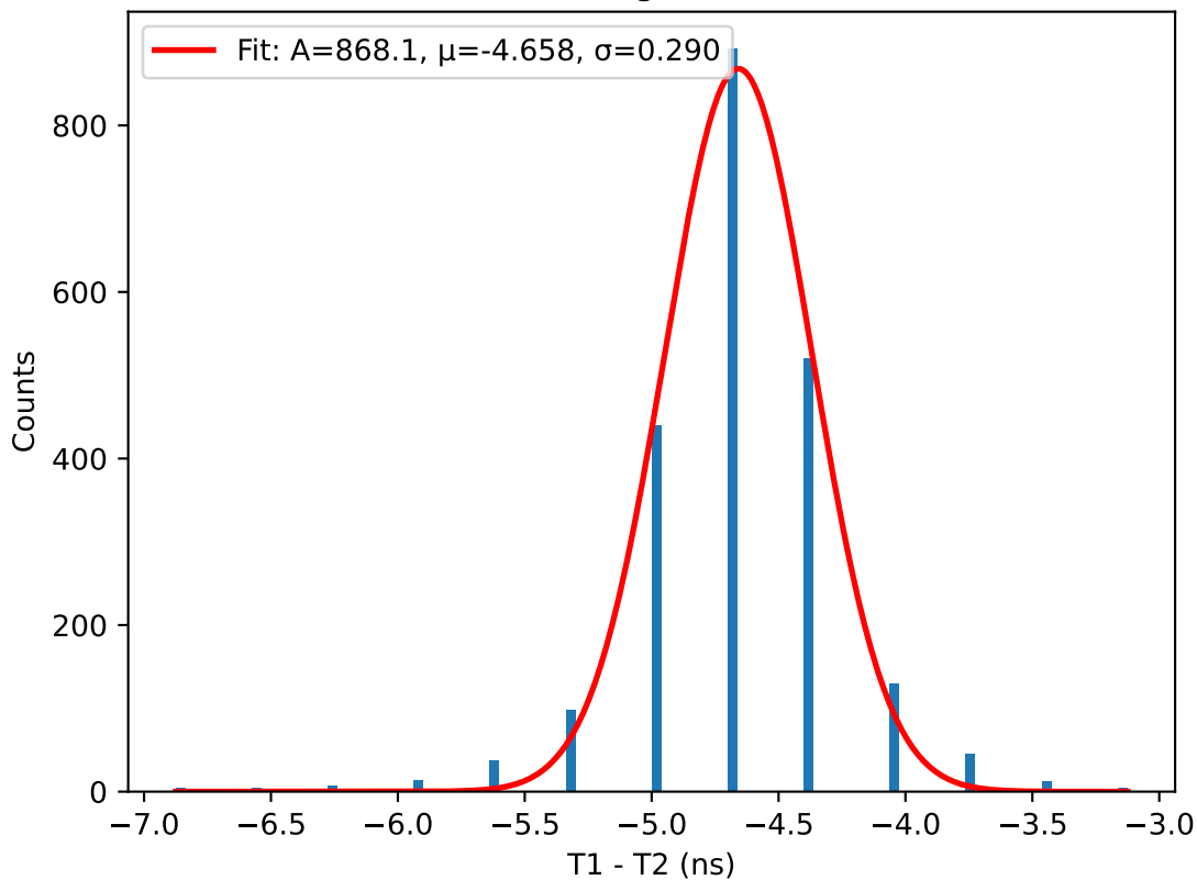
T1 - T2 histogram for 44.0V
