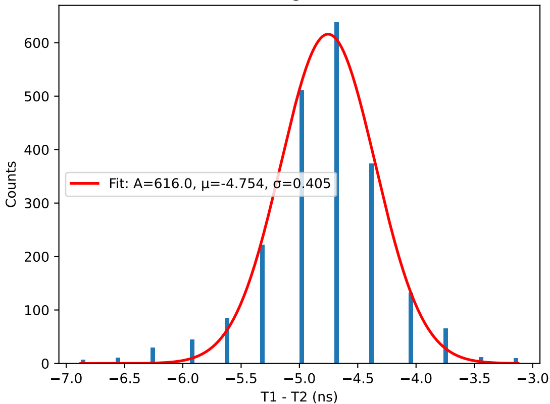
T1 - T2 histogram for 41.5V
