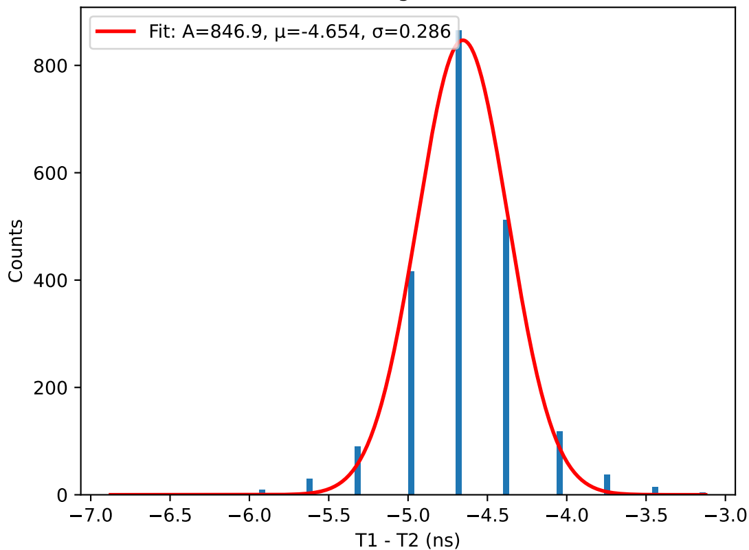
T1 - T2 histogram for 44.5V
